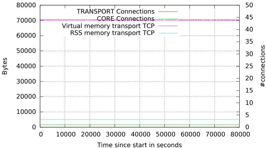
Resource consumption with HTTP and HTTPS plugin
