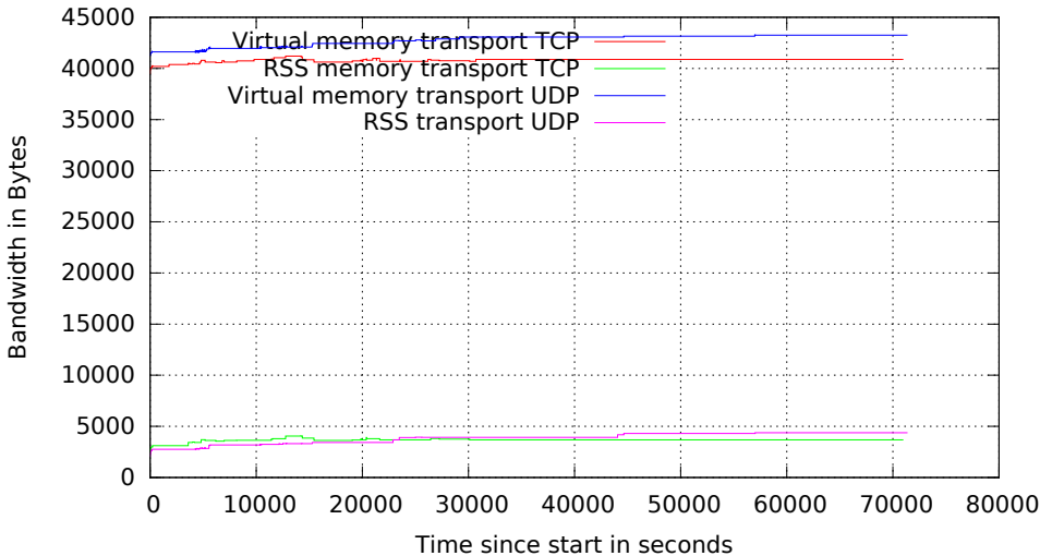
Memory consumption in Bytes, 1 plugin enabled
